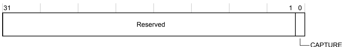
Figure 4-53 GICP_CAPR bit assignments
