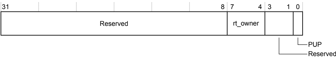
Figure 4-7 GICD_DCHIPR bit assignments
