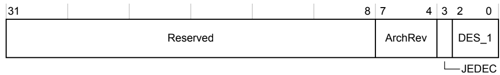
Figure 4-33 GITS_PIDR2 bit assignments
