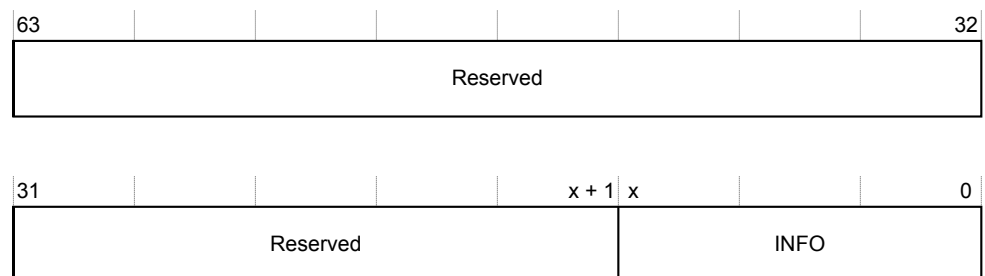
Figure 4-39 GICT_ERR10MISC1 bit assignments
